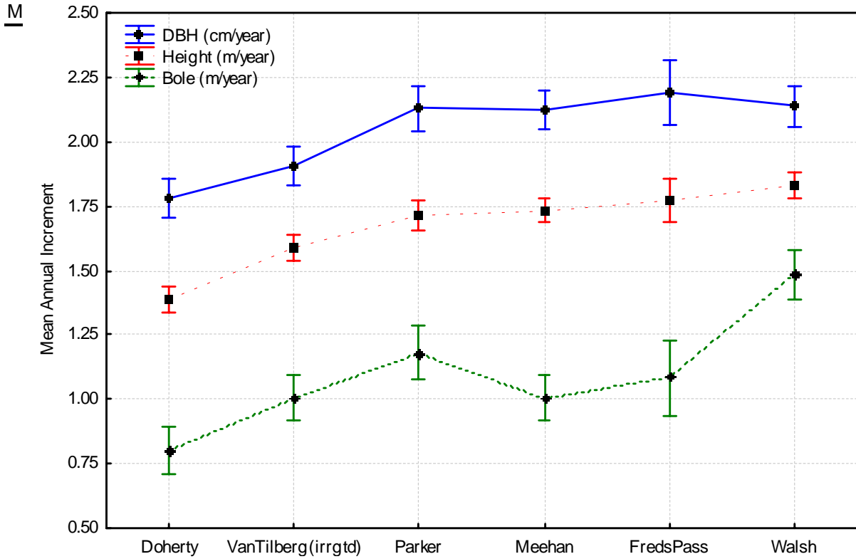
Figure 10 Shows the incremental increases (MAI) for height, diameter and bole length for T. grandis at all sites established 1999/00.
